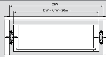
Technical Dimensions
