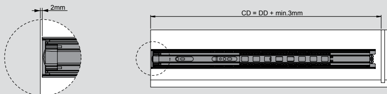
Drawer Dimensions
