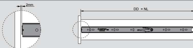
Drawer Dimensions
