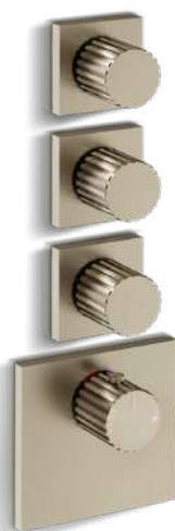
43105_75306 Thermostatic high-capacity mixer with 3 separate exits / Miscelatore termostatico alta portata 3 uscite indipendenti 43103_75304 2 exits / 2 uscite 43107_75308 4 exits / 4 uscite 43109_75310 5 exits / 5 uscite
